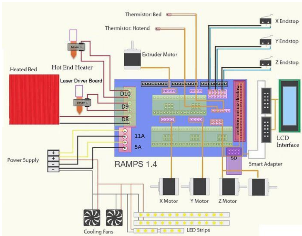
2) The referring wiring schematic diagram of Sanguinololu
